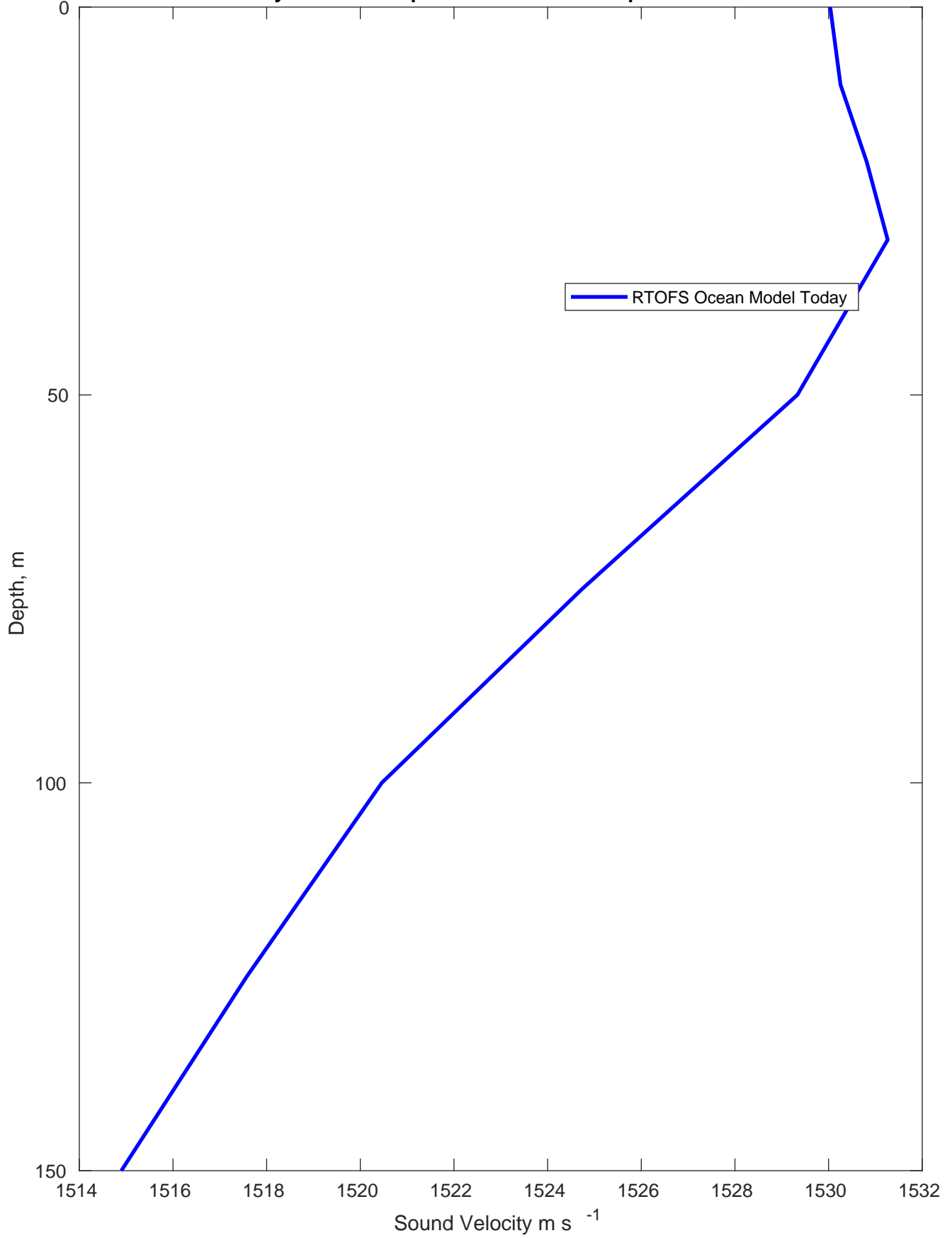
Sound Velocity Profile for Apache VK 694 on 21-Apr-2022 00:00:00
